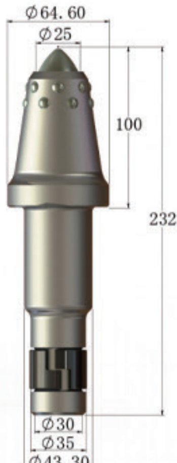
GL100 43(35)-U170 Z2535E14-C(RS1)
