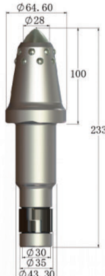
GL100 43(35)-U170 S2837E14-C(RS1)
