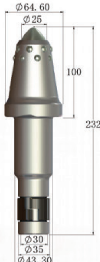
GL100 43(35)-U170 S2535E14-C(RS1)
